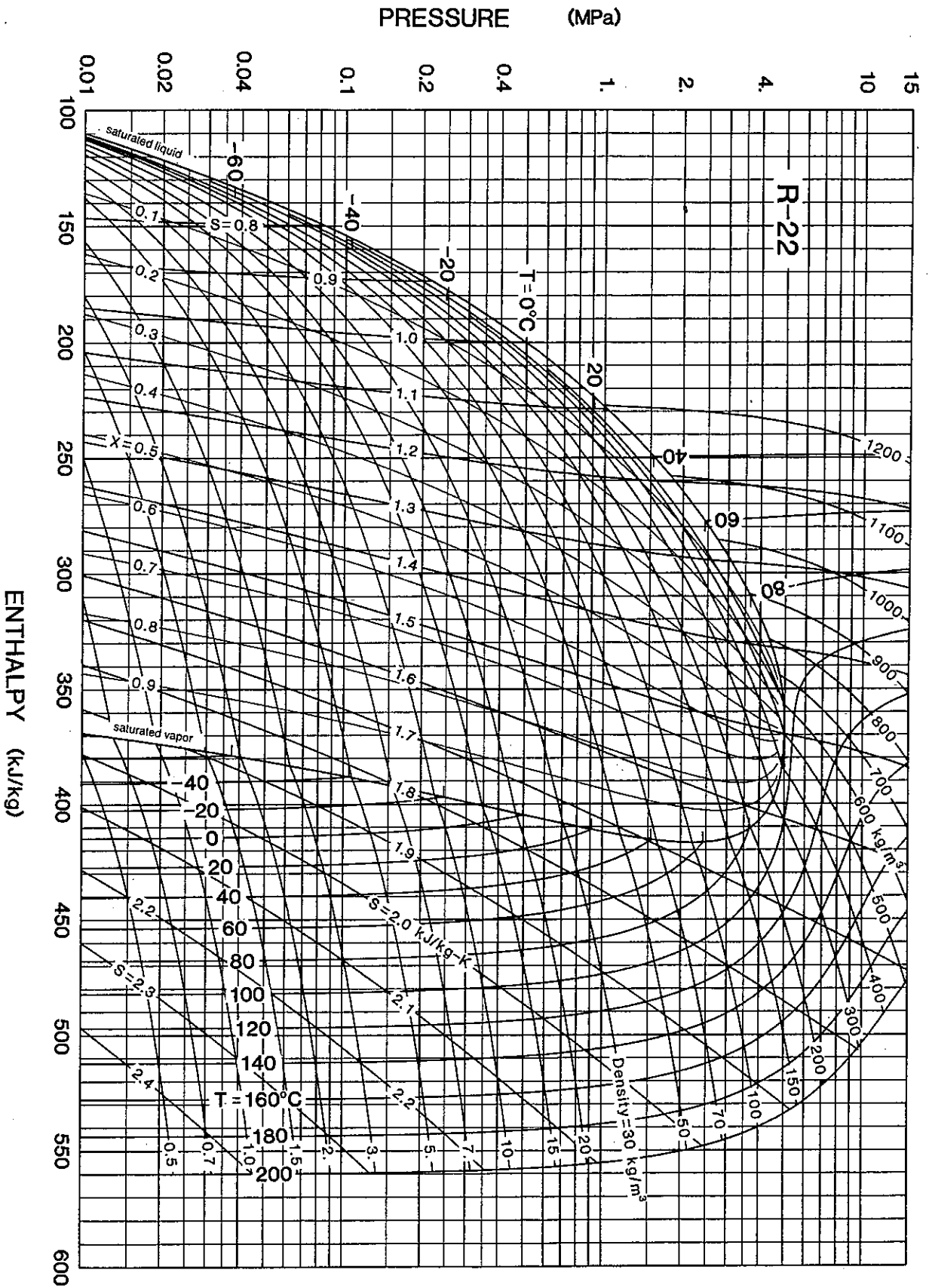
Fig. 4 Pressure-Enthalpy Diagram for Refrigerant 22
